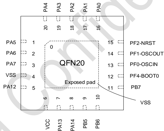
图 3-10 QFN20 Pinout2 PY32F030F2xUx / PY32F030F2xUx-E
