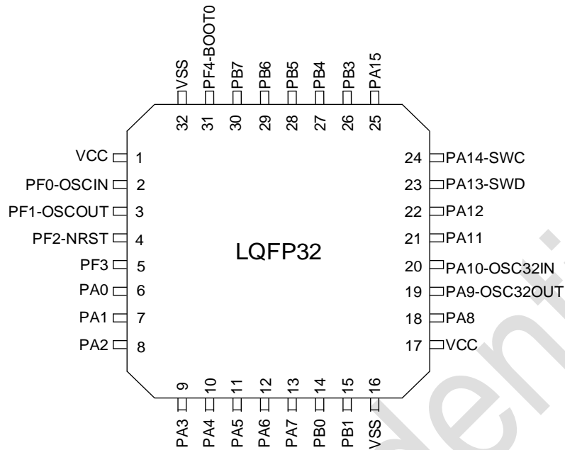
图 3-1 LQFP32 Pinout1 PY32F030K1xTx
